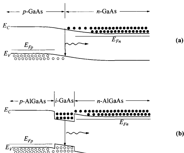
Fig. 9 (a) Under forward bias of a p - n junction, electrons injected from n -side recombine with holes injected from p -side. (b) Higher carrier densities and improved carrier confinement in a double heterojunction.
