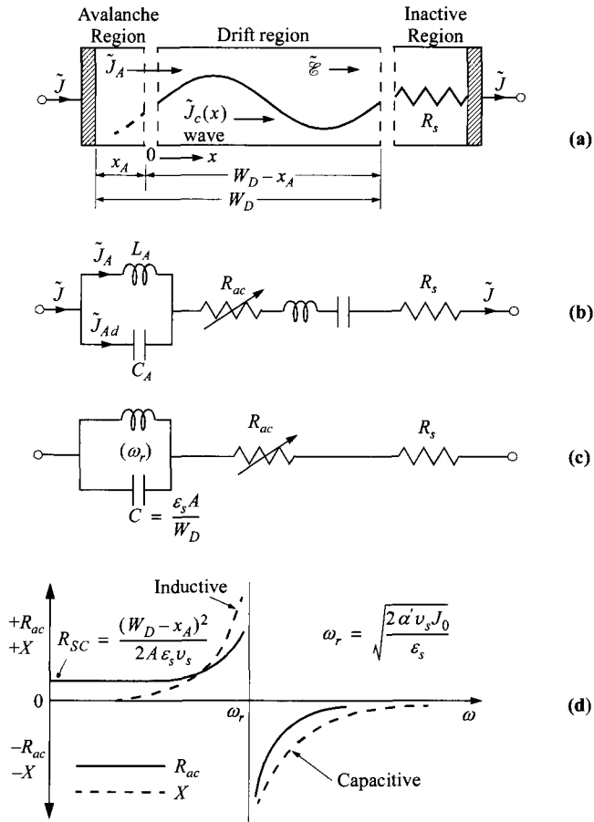
Fig. 7 (a) Model of Read diode with avalanche, drift, and inactive regions, and (b) its equivalent circuit. For small transit angle \theta_p , (c) equivalent circuit and (d) plots of real and imaginary parts of impedance vs. angular frequency \omega (After Ref. 7.)
