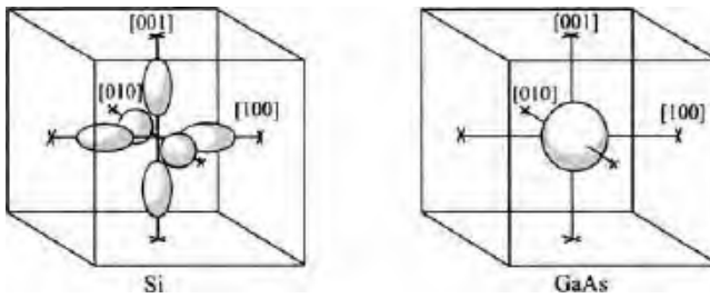
Fig. 5 Shapes of constant-energy surfaces for electrons in Si and GaAs. For Si there are six ellipsoids along the \langle 100 \rangle -axes with the centers of the ellipsoids located at about three-fourths of the distance from the Brillouin zone center. For GaAs the constant energy surface is a sphere at zone center. (After Ref. 21.)
