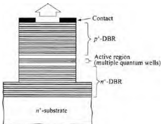
Fig. 46 Structure of vertical-cavity surface-emitting laser (VCSEL).
