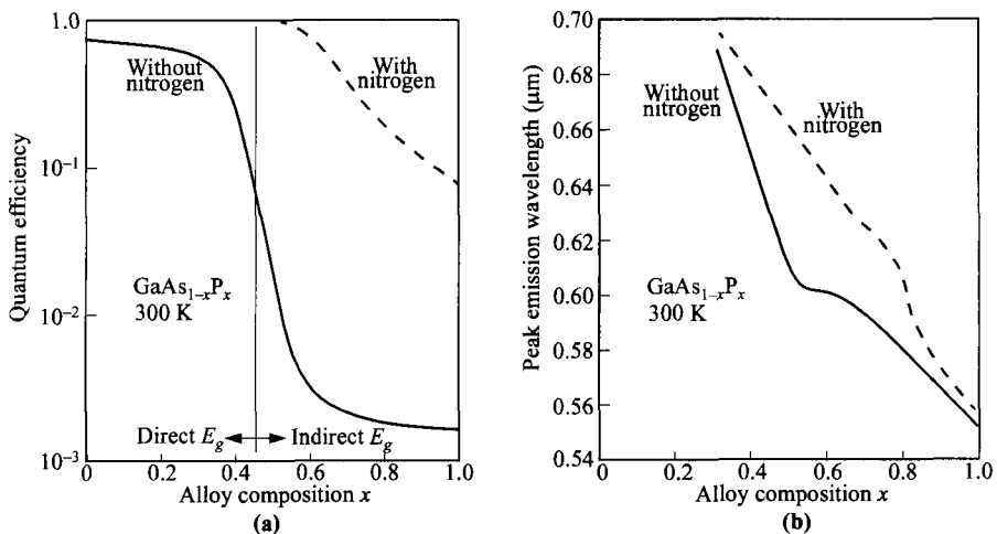
Fig. 12 (a) Quantum efficiency of GaAs 1-x P x vs. alloy composition, with and without isoelectronic impurity nitrogen. (b) Peak emission wavelength vs. composition. (After Ref. 22.)
