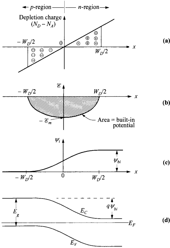
Fig. 5 Linearly graded junction in thermal equilibrium. (a) Space-charge distribution. (b) Electric-field distribution. (c) Potential distribution. (d) Energy-band diagram.
