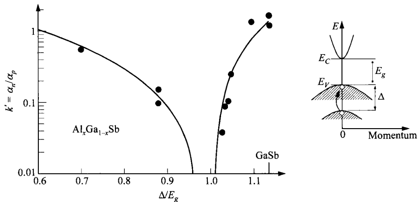
Fig. 20 Ratio of ionization rates in \text{Al}_x\text{Ga}_{1-x}\text{Sb} vs. \Delta/E_g , where \Delta is the spin-orbit splitting of the valence bands shown in the inset. (After Ref. 32.)
