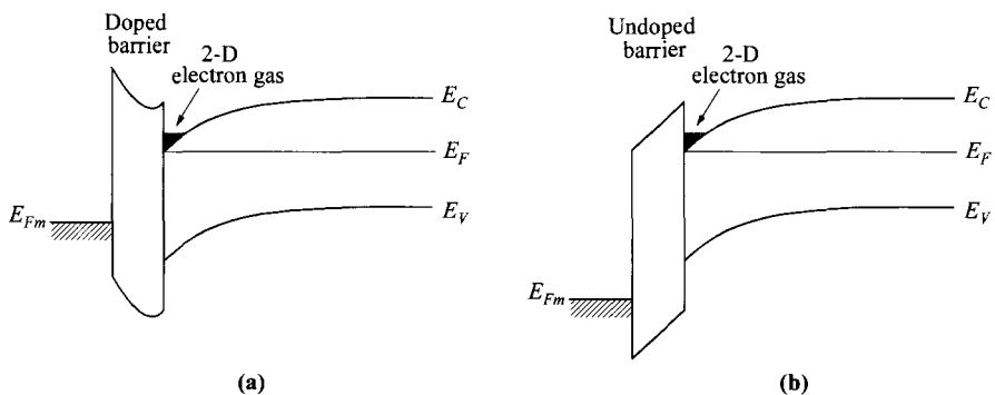
Fig. 22 Comparison of (a) doped barrier layer (as in MODFET) and (b) undoped barrier layer (as in HIGFET), for the same amount of channel charge.
