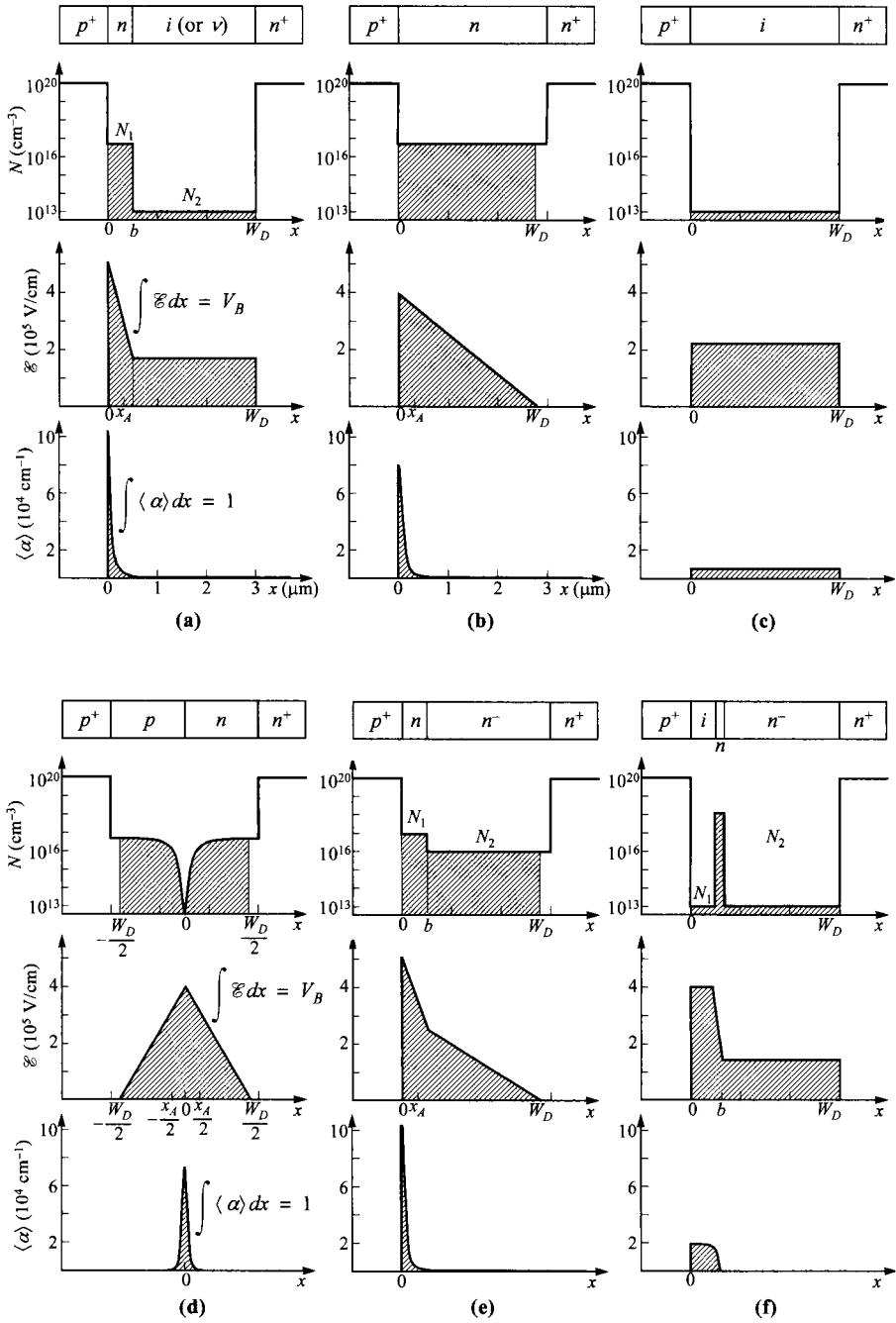
Fig. 1 Doping profile, electric-field distribution, and ionization integrand for (a) Read diode; (b) one-sided abrupt diode; (c) p - i - n diode; (d) double-drift diode; (e) hi-lo structure; and (f) lo-hi-lo structure.
