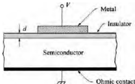
Fig. 1 Metal-insulator-semiconductor (MIS) capacitor, in its simplest form.
