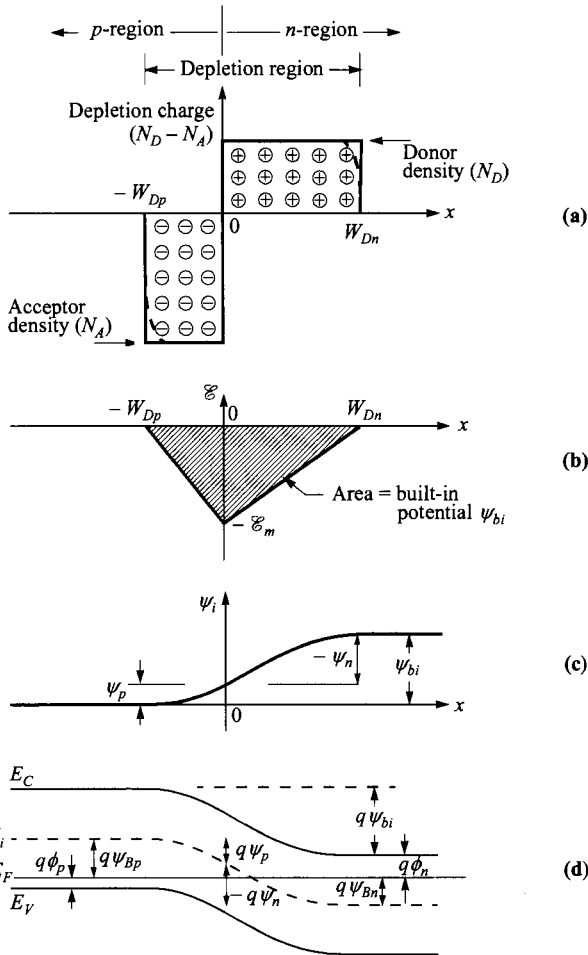
Fig. 1 Abrupt p-n junction in thermal equilibrium. (a) Space-charge distribution. Dashed lines indicate corrections to depletion approximation. (b) Electric-field distribution. (c) Potential distribution where \psi_{bi} is the built-in potential. (d) Energy-band diagram.
