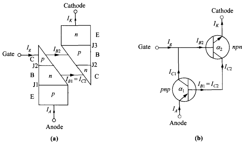
Fig. 8 (a) Two-transistor approximation of a three-terminal thyristor, bisected into (but connected) p - n - p and n - p - n bipolar transistors. (b) Its circuit representation using transistor notations.
