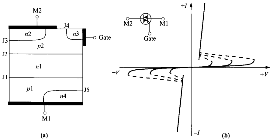
Fig. 23 (a) Cross-section view of a triac, a six-layer structure having five p - n junctions (J1-J5) and three electrode shorts. (b) Triac I - V characteristics for varying gate biases and the device symbol (inset).
