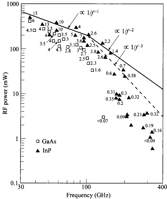
Fig. 17 Output microwave power vs. frequency for cw-operated GaAs and InP TEDs. Numbers next to symbols denote dc-to-RF conversion efficiencies in percentage. (After Ref. 45.)
