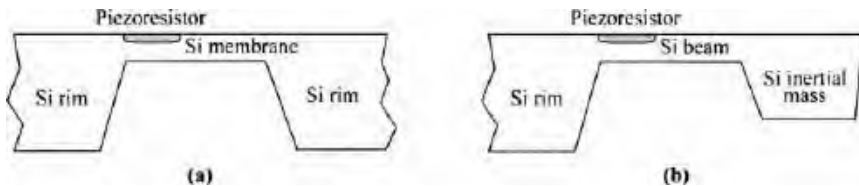
Fig. 6 Sensors based on piezoresistance. (a) Si pressure sensor and (b) acceleration sensor. (After Ref. 1.)
