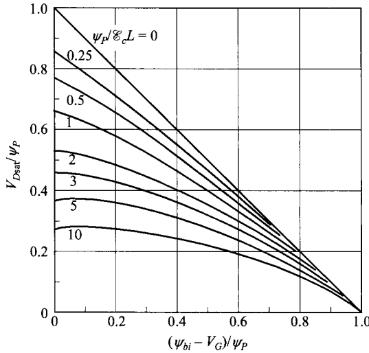
Fig. 5 Solution of V_{Dsat} from Eq. 33, for various values of \psi_P/\mathcal{E}_c L . (After Ref. 6.)
