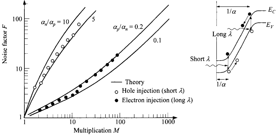
Fig. 14 Experimental results of noise factors for a silicon APD with 0.1- \mu A primary current of two wavelengths. Inset shows energy-band diagram with an electron or hole primary current, depending on the wavelength of the incident light. (After Ref. 21.)
