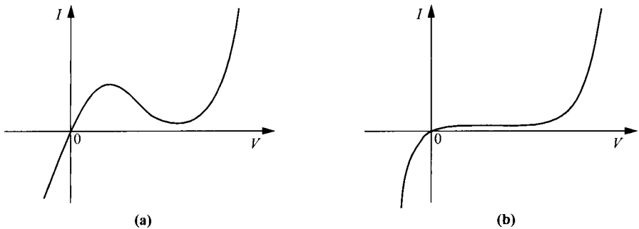
Fig. 15 Comparison of (a) tunnel diode with negative resistance and (b) backward diode without negative resistance.
