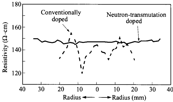
Fig. 4 Comparison of doping uniform of high-resistivity Si by conventional doping and neutron-transmutation doping. (After Ref. 14.)
