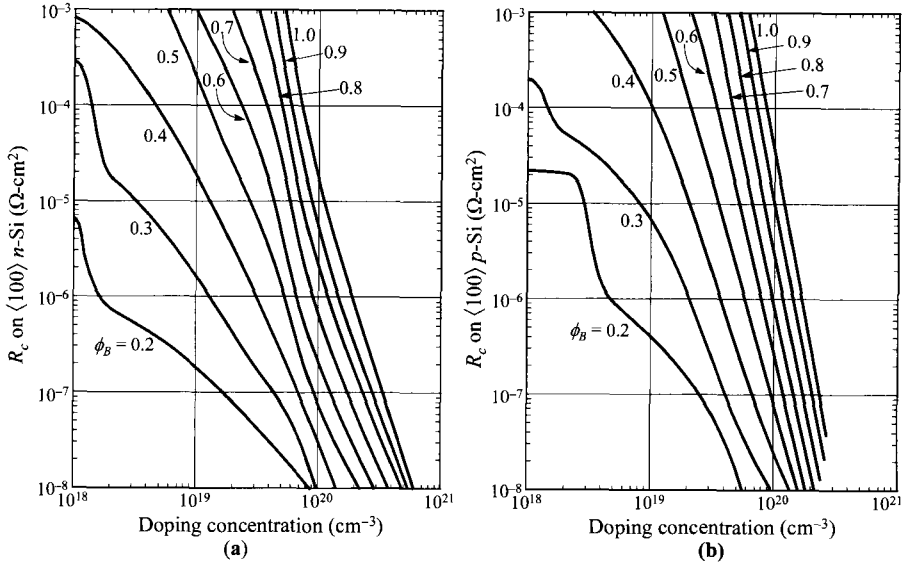
Fig. 40 Calculated specific contact resistance R_c on (a) n -type and (b) p -type \langle 100 \rangle Si surfaces for various barrier heights (in eV) at room temperature. (After Ref. 86)
