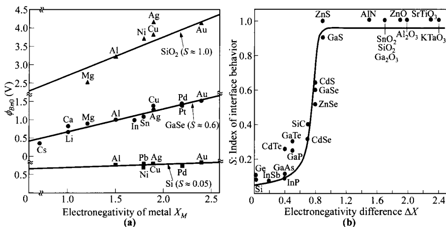
Fig. 8 (a) Barrier height versus electronegativity of metals deposited on Si, GaSe, and SiO 2 . (b) Index of interface behavior S as a function of the electronegativity difference of the semi-conductors. (After Ref. 21.)
