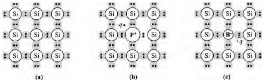
Fig. 7 Three basic bond pictures of a semiconductor. (a) Intrinsic Si with no impurity. (b) n -type Si with donor (phosphorus). (c) p -type Si with acceptor (boron).
