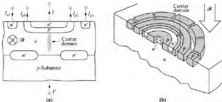
Fig. 21 (a) Carrier-domain magnetometer. Under a magnetic field, the carrier domain shifts laterally, and the current differences I_{p1} - I_{p2} and I_{n1} - I_{n2} are detected. (b) Horizontal, circular carrier-domain magnetometer. The carrier domain rotates with a frequency proportional to magnetic field. (After Ref. 8.)
