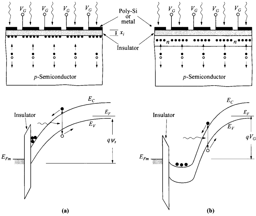
Fig. 23 Structures and energy-band diagrams of (a) surface-channel CCD and (b) buried-channel CCD. For p -type substrate, a positive gate bias is applied to drive the semiconductor into deep depletion under nonequilibrium condition.
