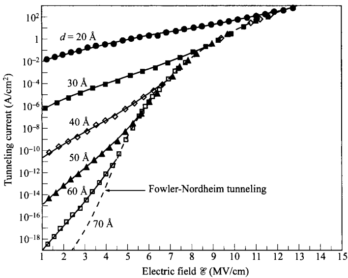
Fig. 18 Tunneling current vs. field for different oxide thicknesses. For thicker oxides Fowler-Nordheim tunneling dominates and is independent of thickness. Direct tunneling occurs in thinner oxides at low fields. (After Ref. 42.)
