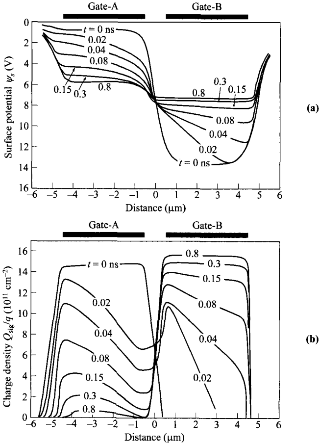
Fig. 30 (a) Time-dependent surface potential distribution under the storage and transfer gate (of length 4\text{-}\mu\text{m} ). (b) Transient charge distribution under the gates. (After Ref. 48.)
