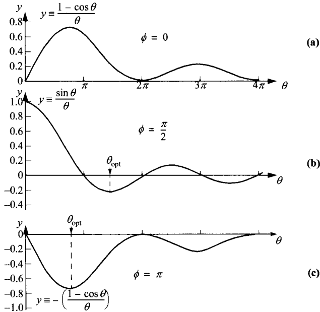
Fig. 6 AC resistance vs. transit angle for three different injection phase delays. (a) \phi = 0 . (b) \phi = \pi/2 . (c) \phi = \pi .
