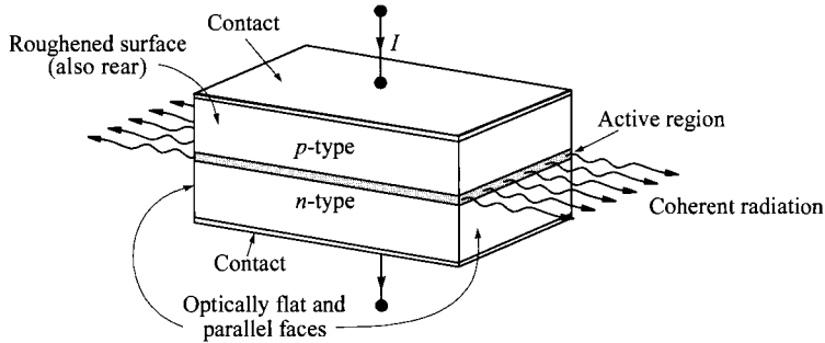
Fig. 24 Basic structure of a junction laser in the form of a Fabry-Perot cavity.
