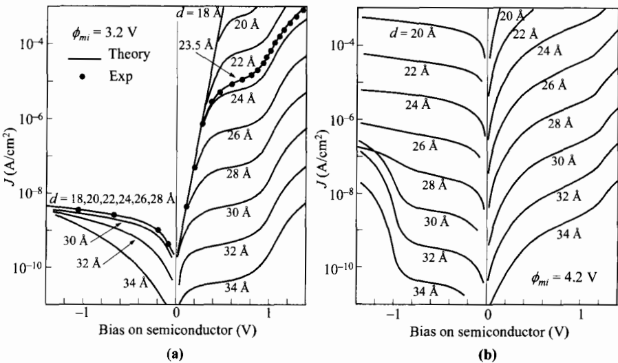
Fig. 22 Current-voltage characteristics of MIS tunnel diodes having: (a) low barrier \phi_{mi} , (b) high barrier. T = 300 K. N_A = 7 \times 10^{15} \text{ cm}^{-3} . (After Ref. 47.)
